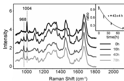
Figure 2. Time-dependent spontaneous Raman spectra of HeLa cells with 80\text{ s} acquisition, showing a decline in the 1004\text{ cm}^{-1} peak and a rise in the 968\text{ cm}^{-1} peak. The valley at 986\text{ cm}^{-1} is used in background subtraction for the SRS images. Inset: single exponential fitting of the ^{12}\text{C}/(^{12}\text{C}+^{13}\text{C}) ratios obtained from the spectra.
